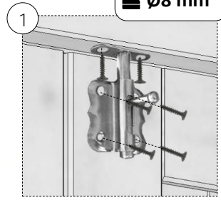
INSIDE Ø3,5x35 (x6)
