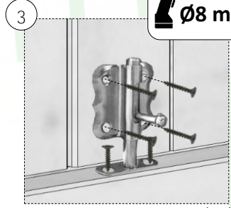
INSIDE Ø3,5x35 (x6)
